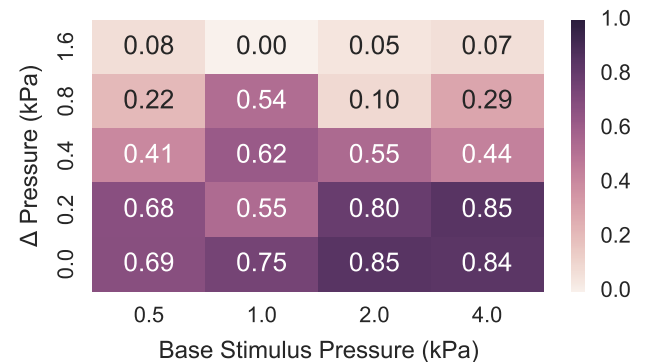
Figure 10. Table showing how often stimulus pairs were judged as being equal (e.g., a 0.8 kPa increase over a 2.0 kPa base pressure was seen as equal only 10 % of the time). This shows that the higher the delta pressure, the more likely a stimulus pair was rated as feeling unequal.
